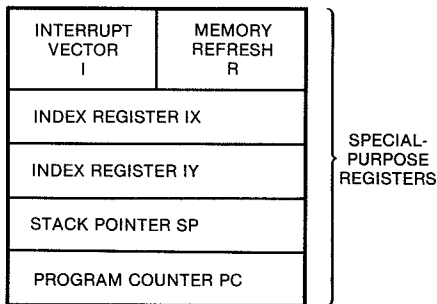
Fig. 4-3. The Z80 register set. (Courtesy MOSTEK Corp.)
